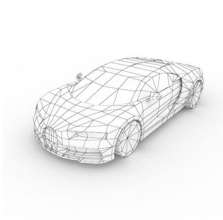
3D mesh
