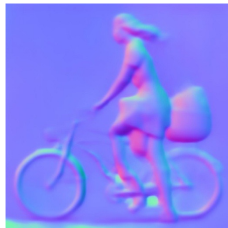
Normal map
