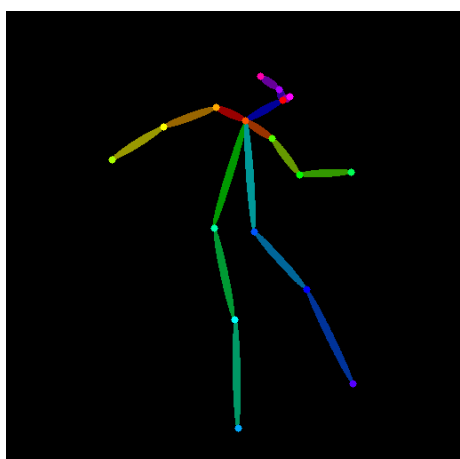
Human pose
