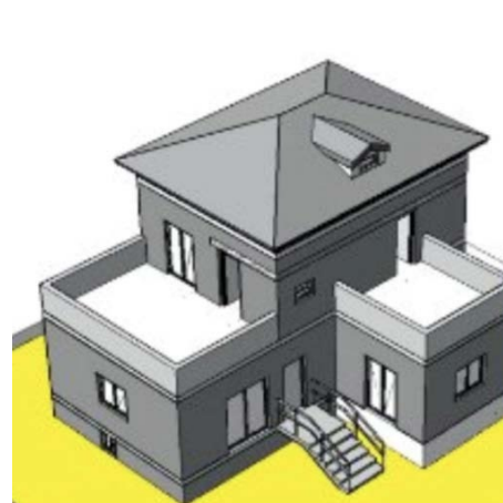
AutoCAD viewport
